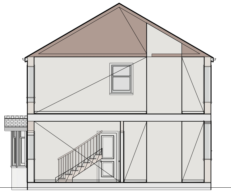
SECOND SIDE ELEVATION (SECTION THROUGH) EXISTING
