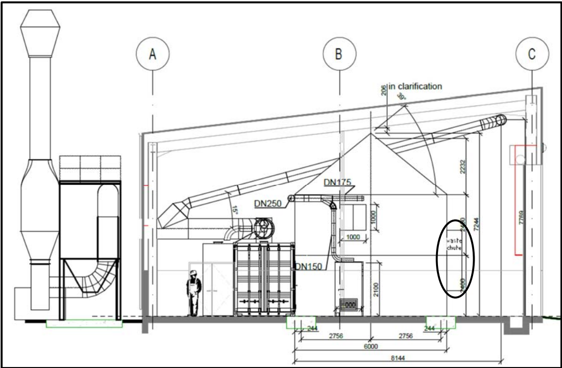
Left Elevation incl. position of waste chute
