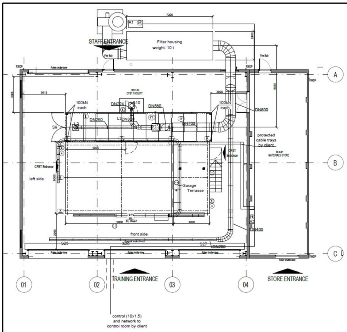
Plan view giraffe building with domestic and demo/attack unit (sectional)
