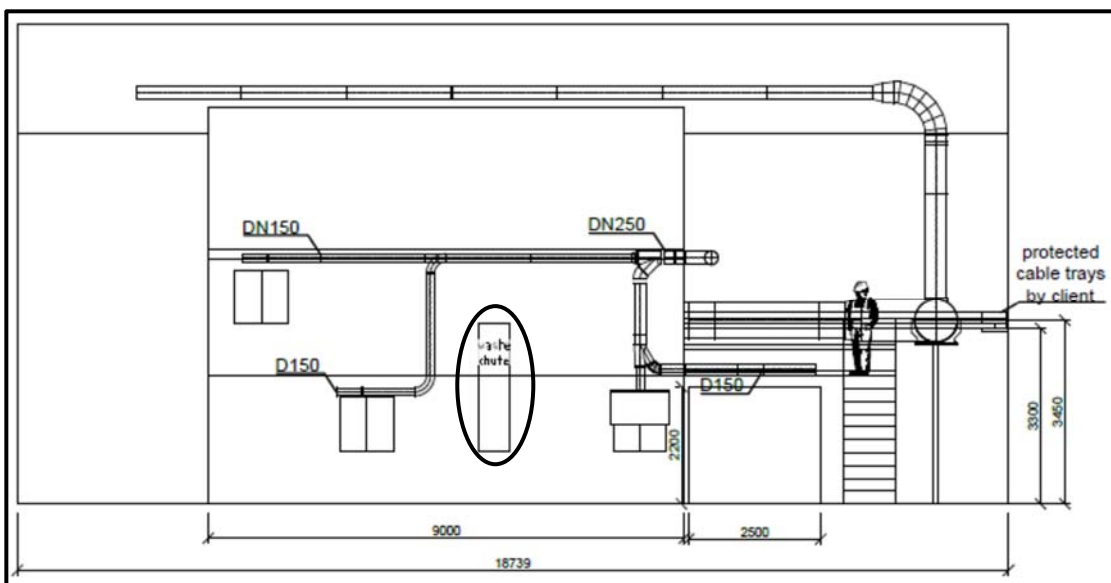
Front Elevation incl. position of waste chute
