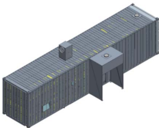
Chimney with lockable flap on the roof of the observation room covered by a special rollover extraction hood (hood made of stainless steel)
