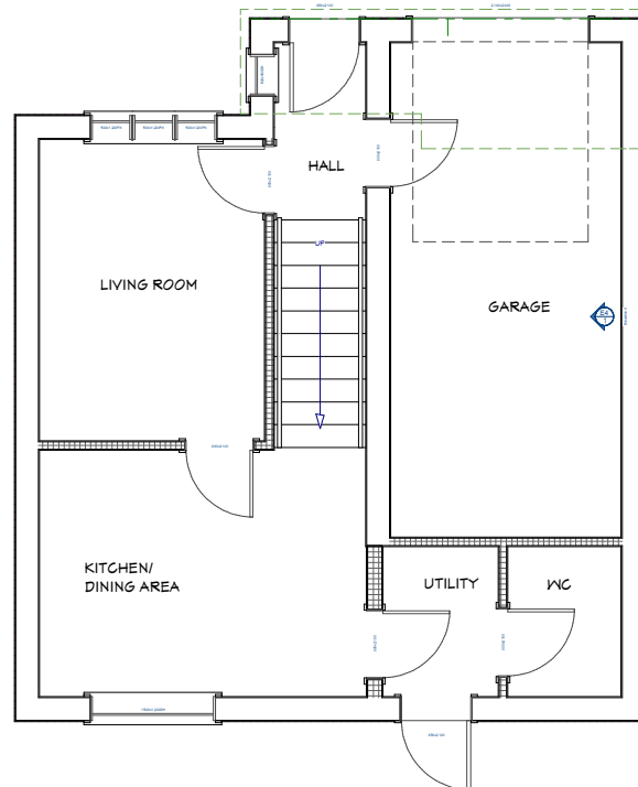
FLOOR PLAN EXISTING
