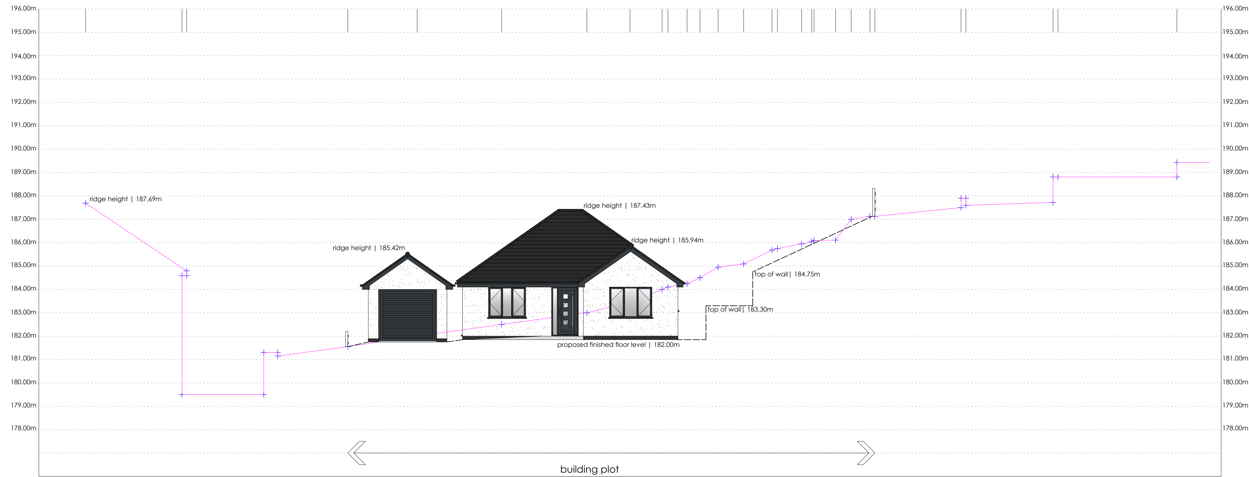
existing-proposed section a-a
