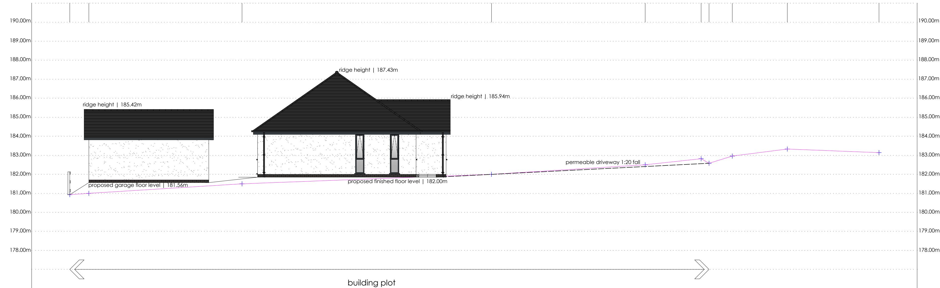
existing-proposed section b-b
