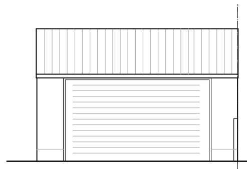
ELEVATION TO LANE SCALE 1:100
