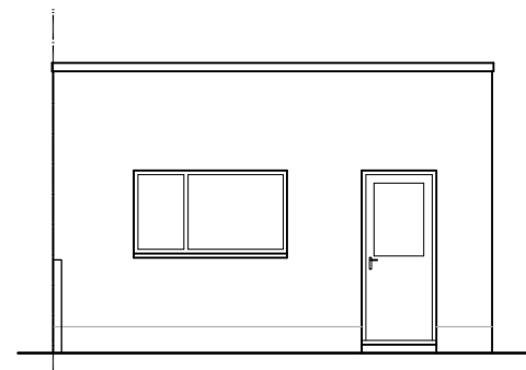
ELEVATION TO HOUSE SCALE 1:100
