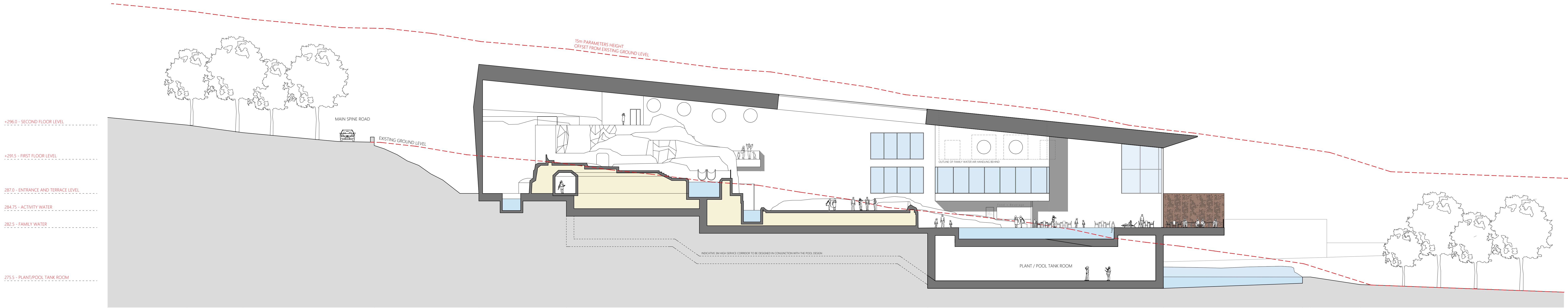
Section 1 1:200
