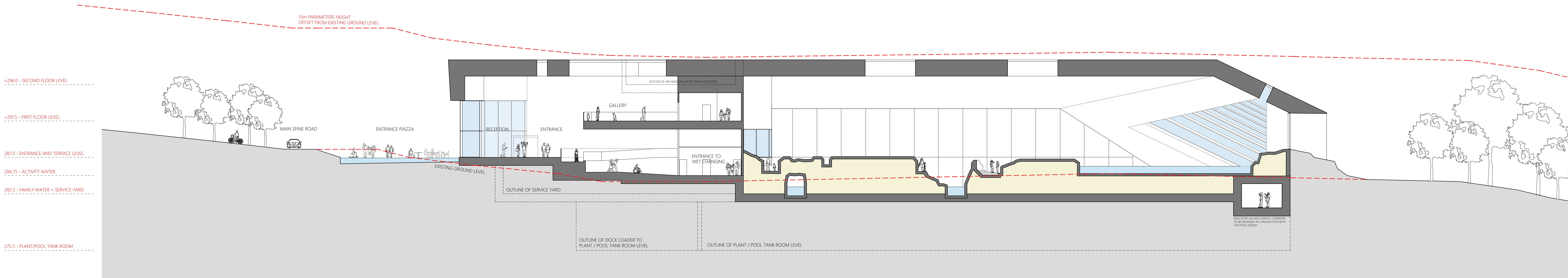
Section 3 1:200
