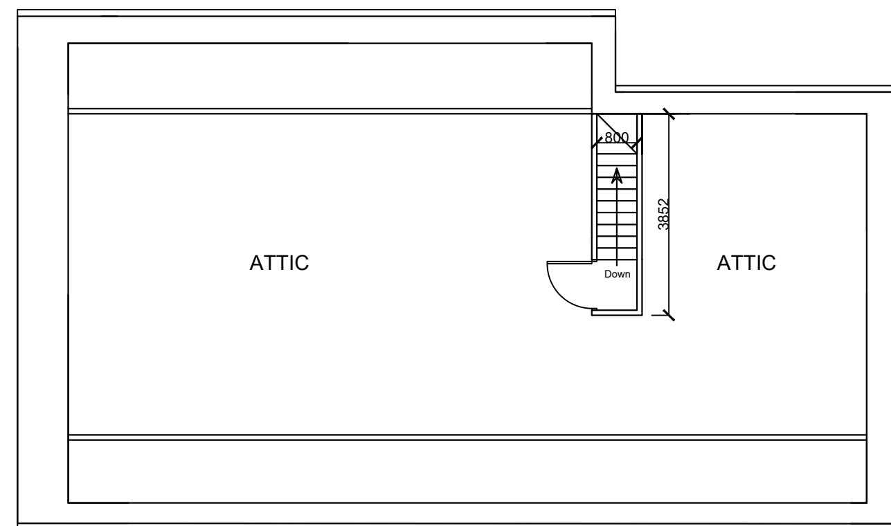
PROPOSED ATTIC FLOOR PLAN
