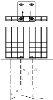
BASEPLATED POSTS (OPTIONAL)
