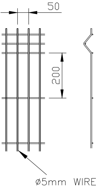
MESH DETAILS
