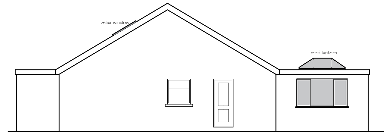
Proposed LH Side Elevation
