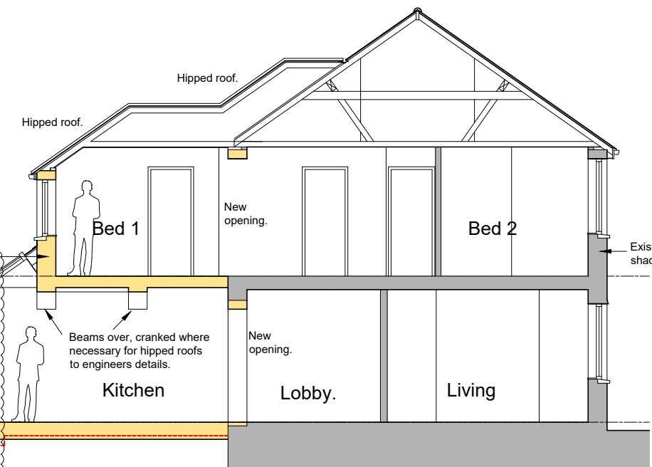
Proposed Section BB 1:100
