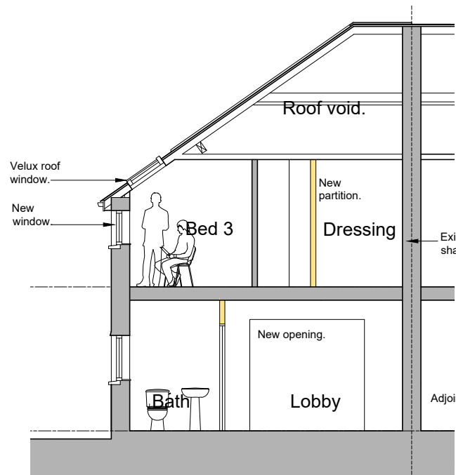
Proposed Section AA 1:100
