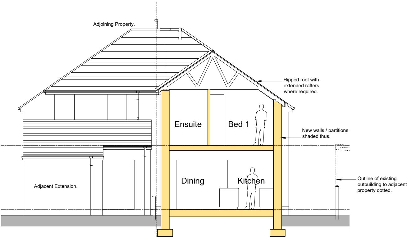
Proposed Section CC 1:100
