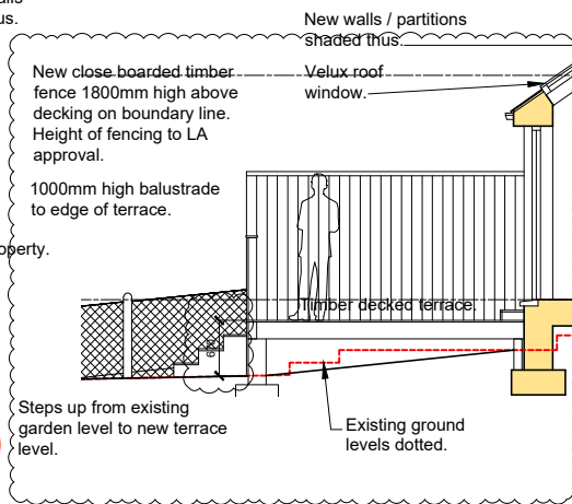
Proposed Section AA 1:100
