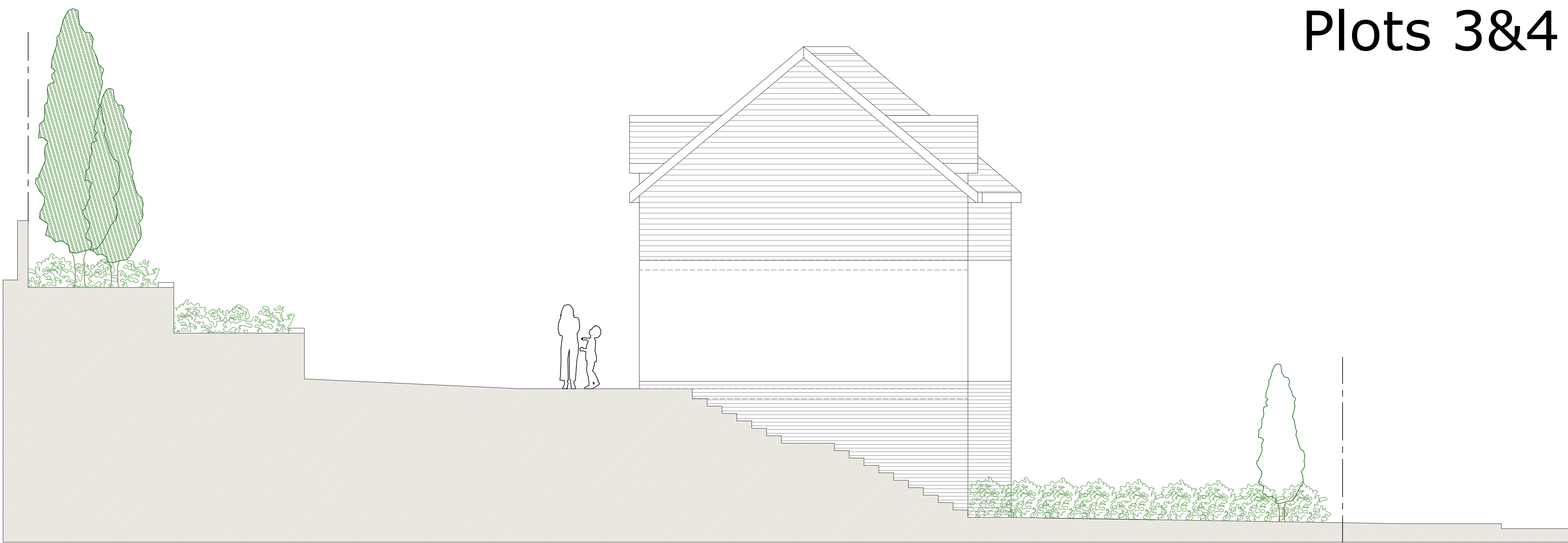
Side Elevation (to plot 3)
