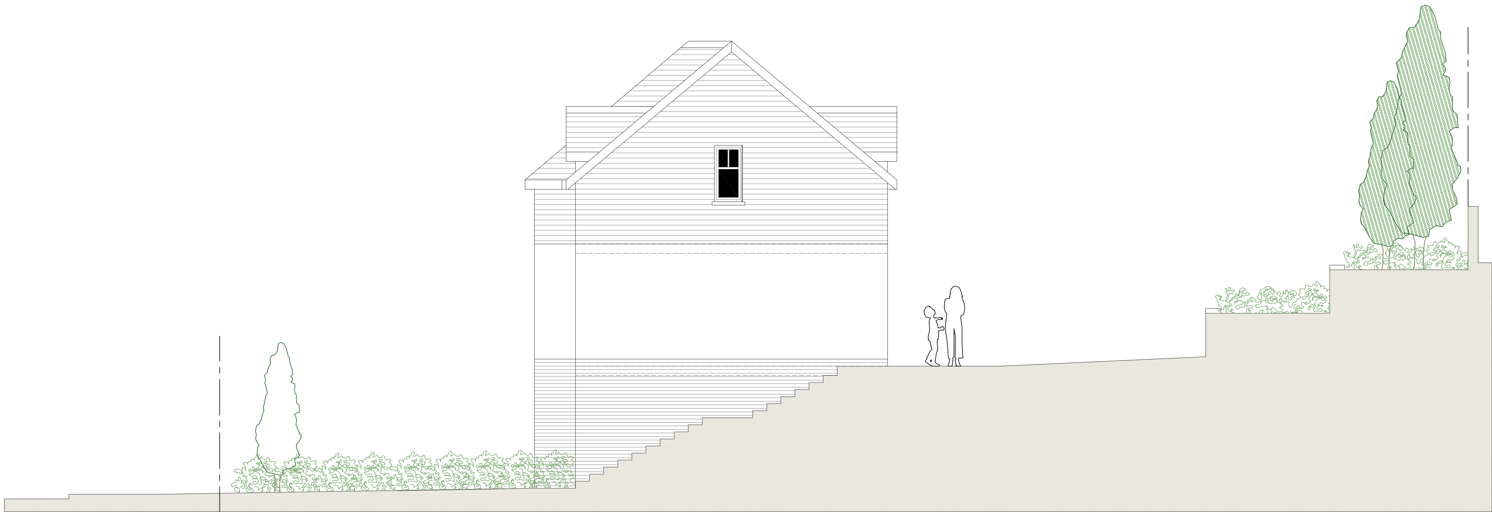
Side Elevation (to plot 4)
