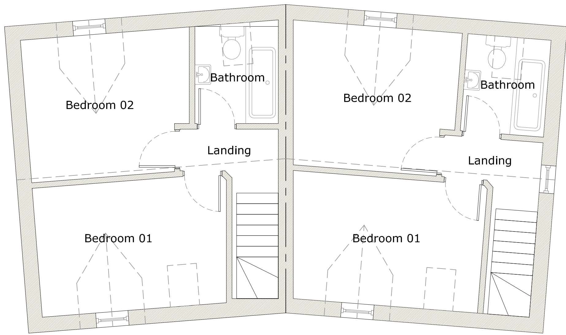
First Floor - 32.0m² (per dwelling to 1.5m high)
