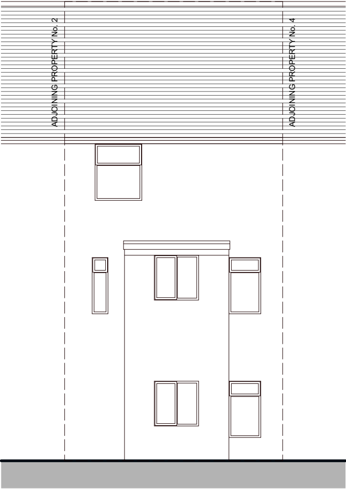
REAR ELEVATION
