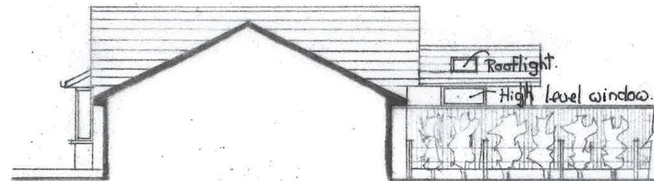
Side Elevation
