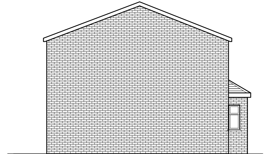
PROPOSED LH SIDE ELEVATION
