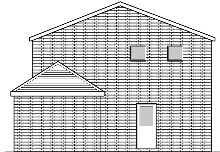
PROPOSED RH SIDE ELEVATION
