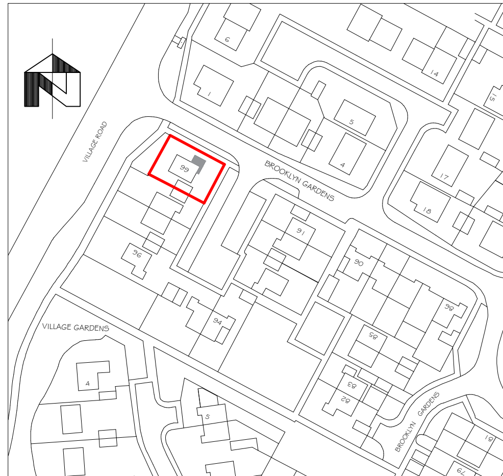
LOCATION PLAN 1:1250
