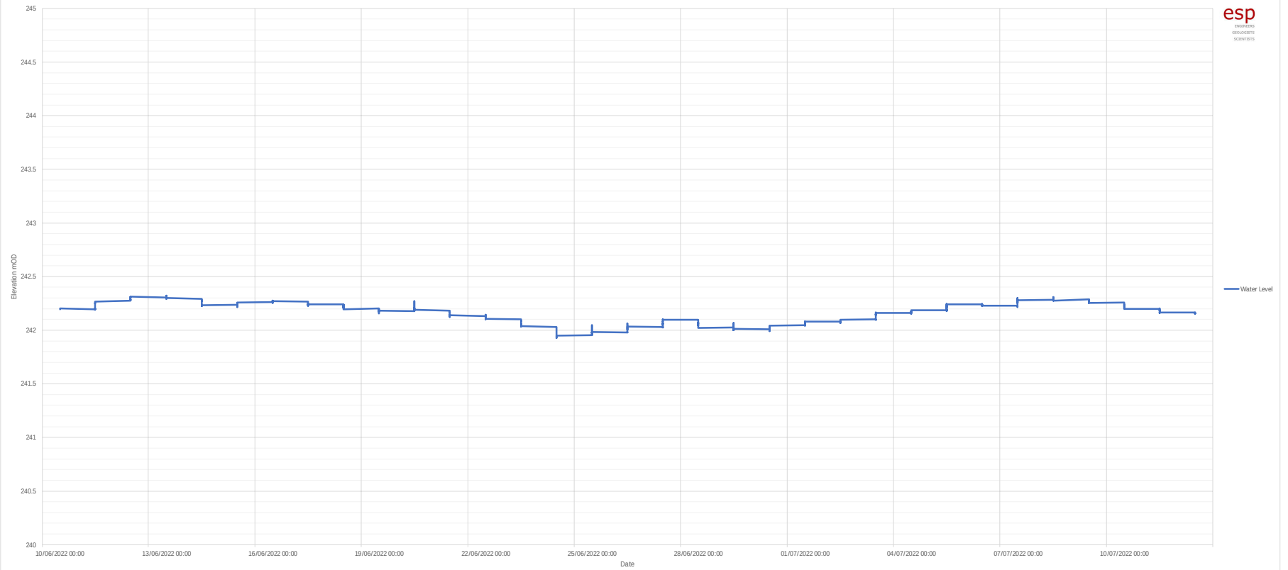
Afan Valley Resort - BH10 - Vibrating Wire Piezometer
