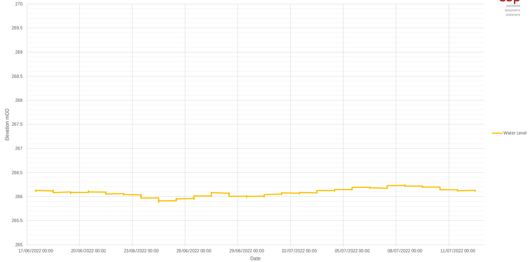
Afan Valley Resort - BH11 - Vibrating Wire Piezometer
