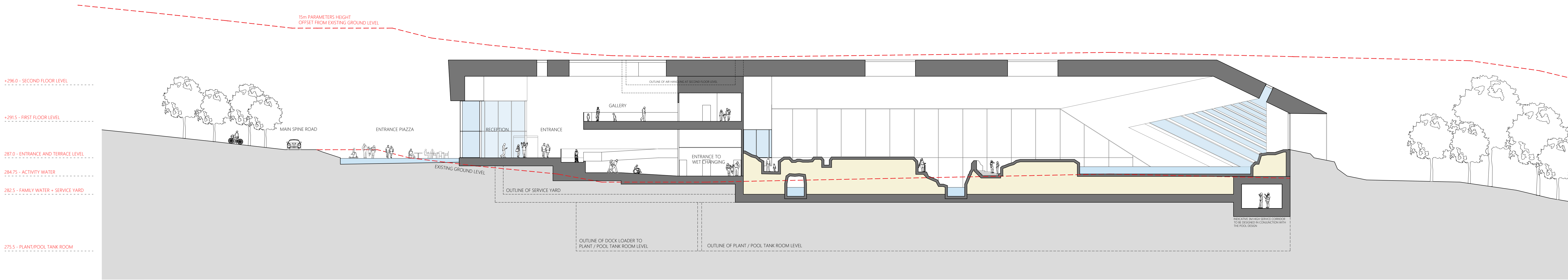
Section 3 1:200
