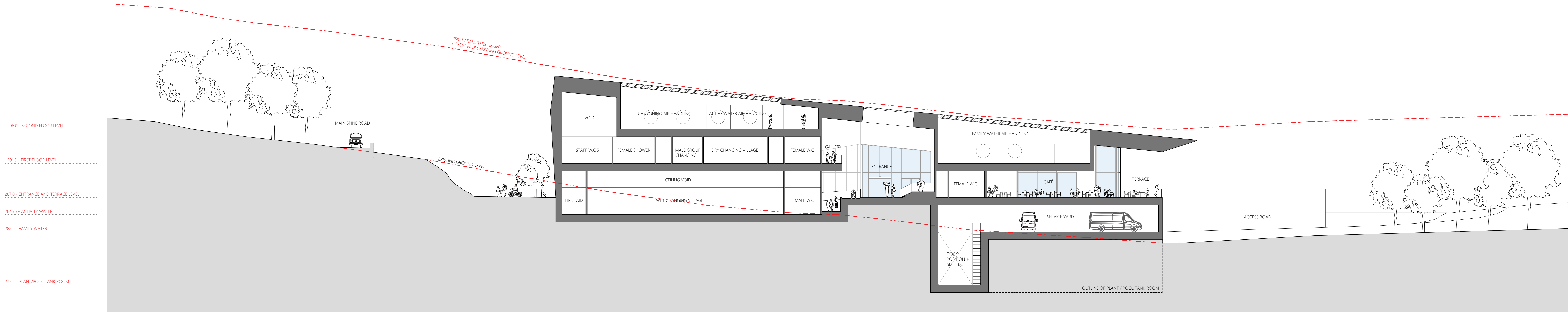
Section 2 1:200
