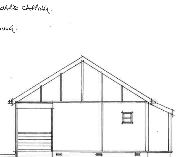
NORTH ELEVATION
