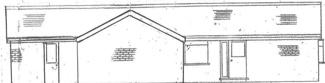
Left hand side Elevation Proposed REVISED
