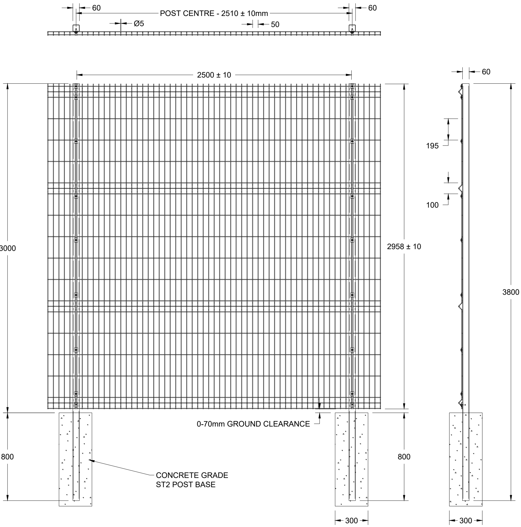
3.0m HIGH V-MESH FENCING SCALE - 1:20
