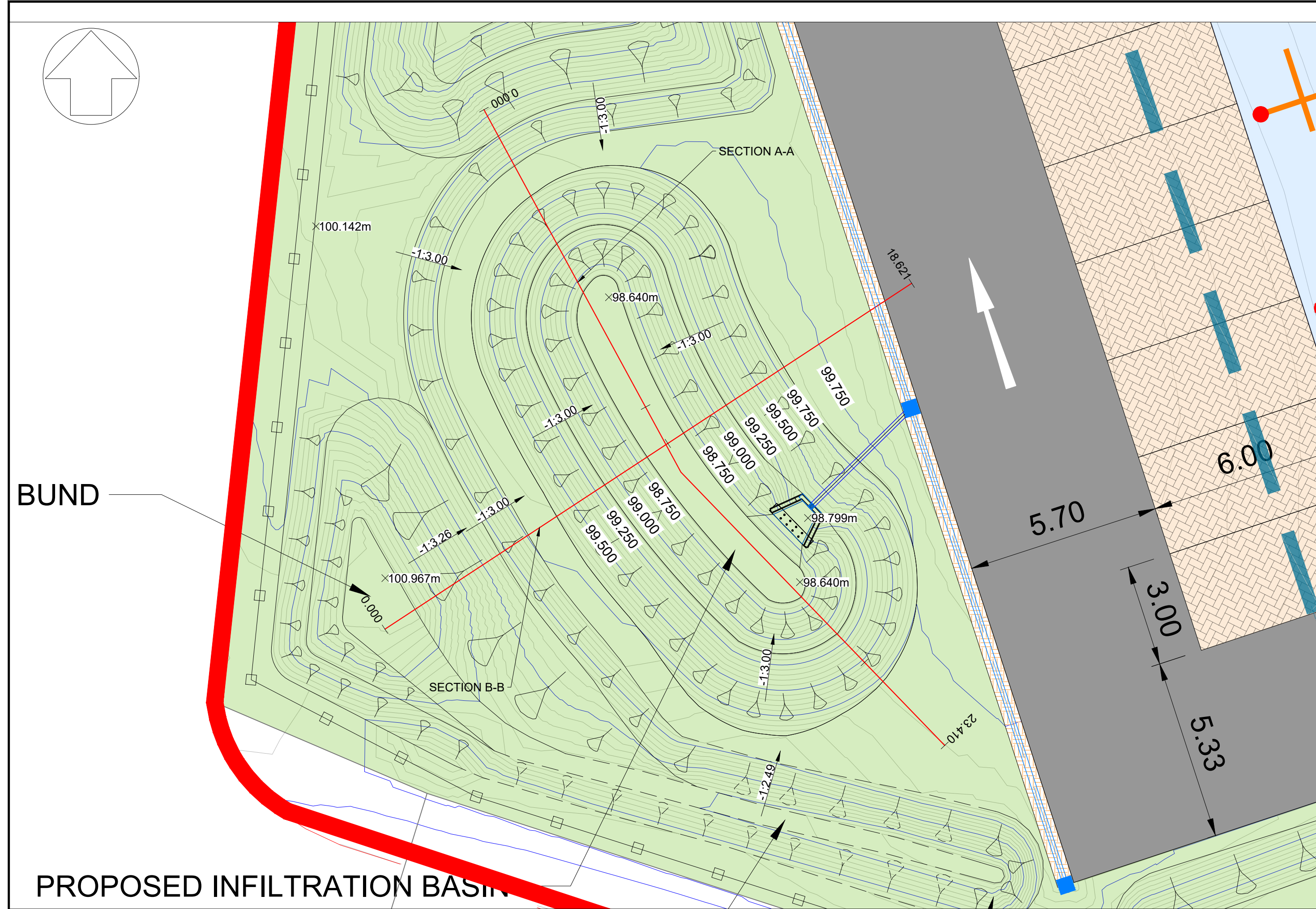
POND GENERAL ARRANGEMENT SCALE - 1:100
