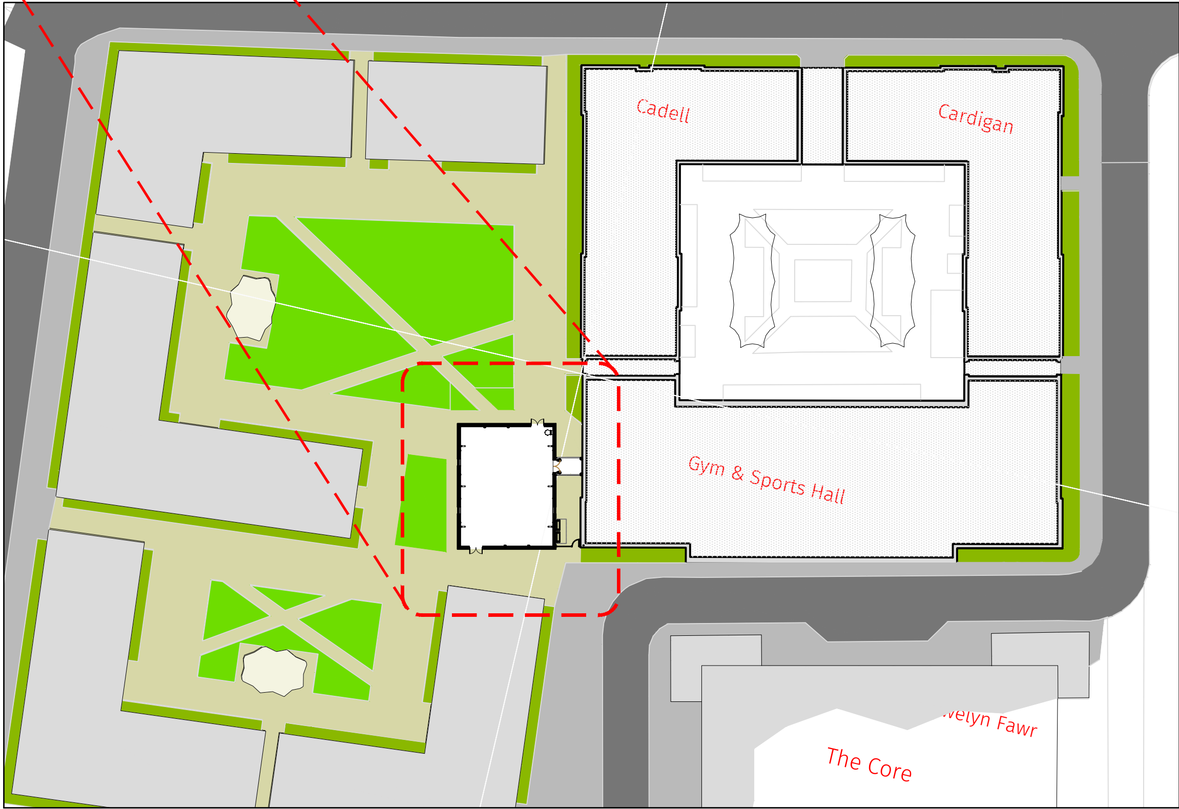
2 PROPOSED GYM & SPORTS HALL BUILDING 1/500@A1
