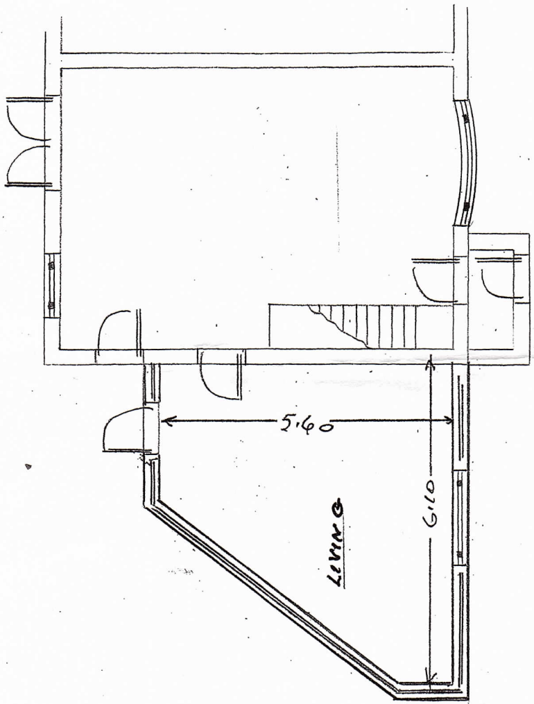
GROUND FLOOR EXISTING AND PROPOSED
