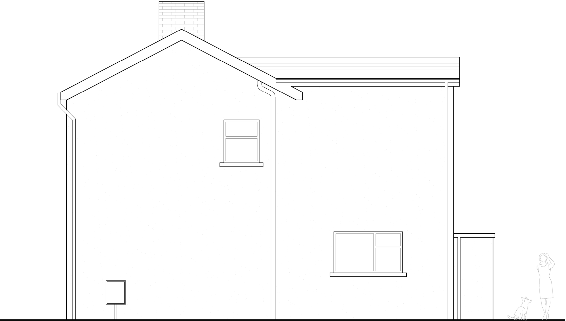
Side (East) Elevation
