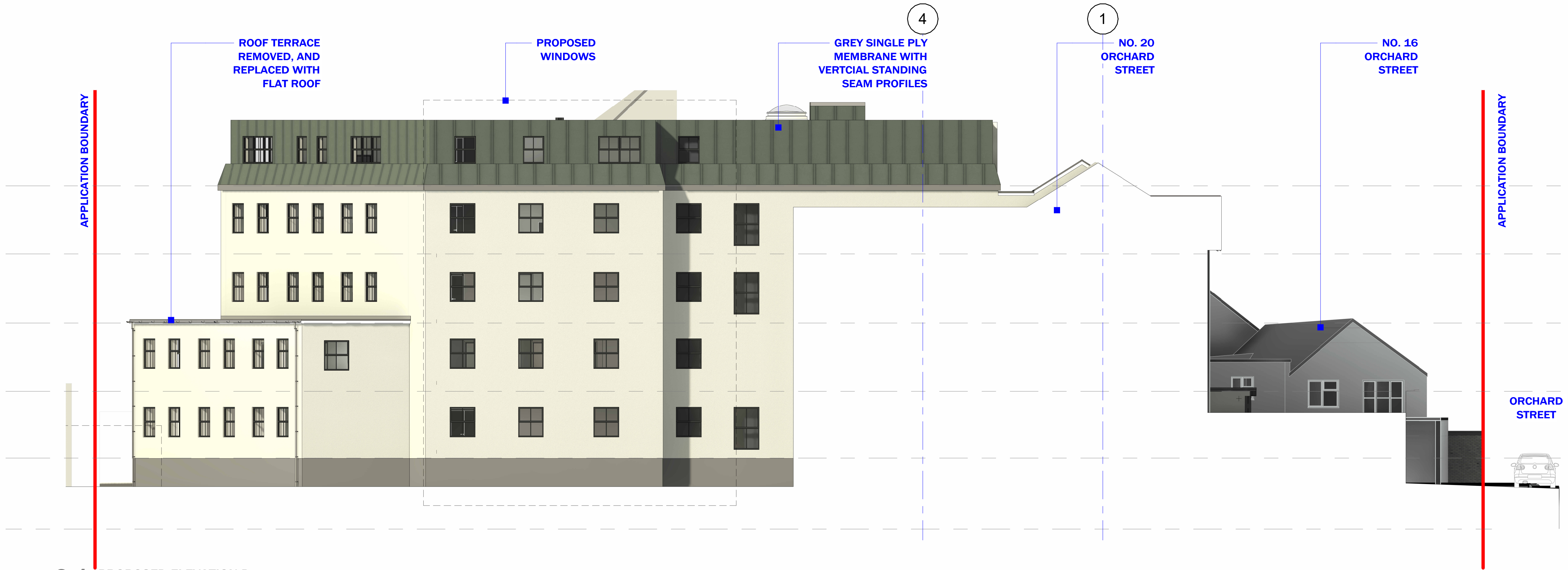
01 PROPOSED ELEVATION D 1 : 100
