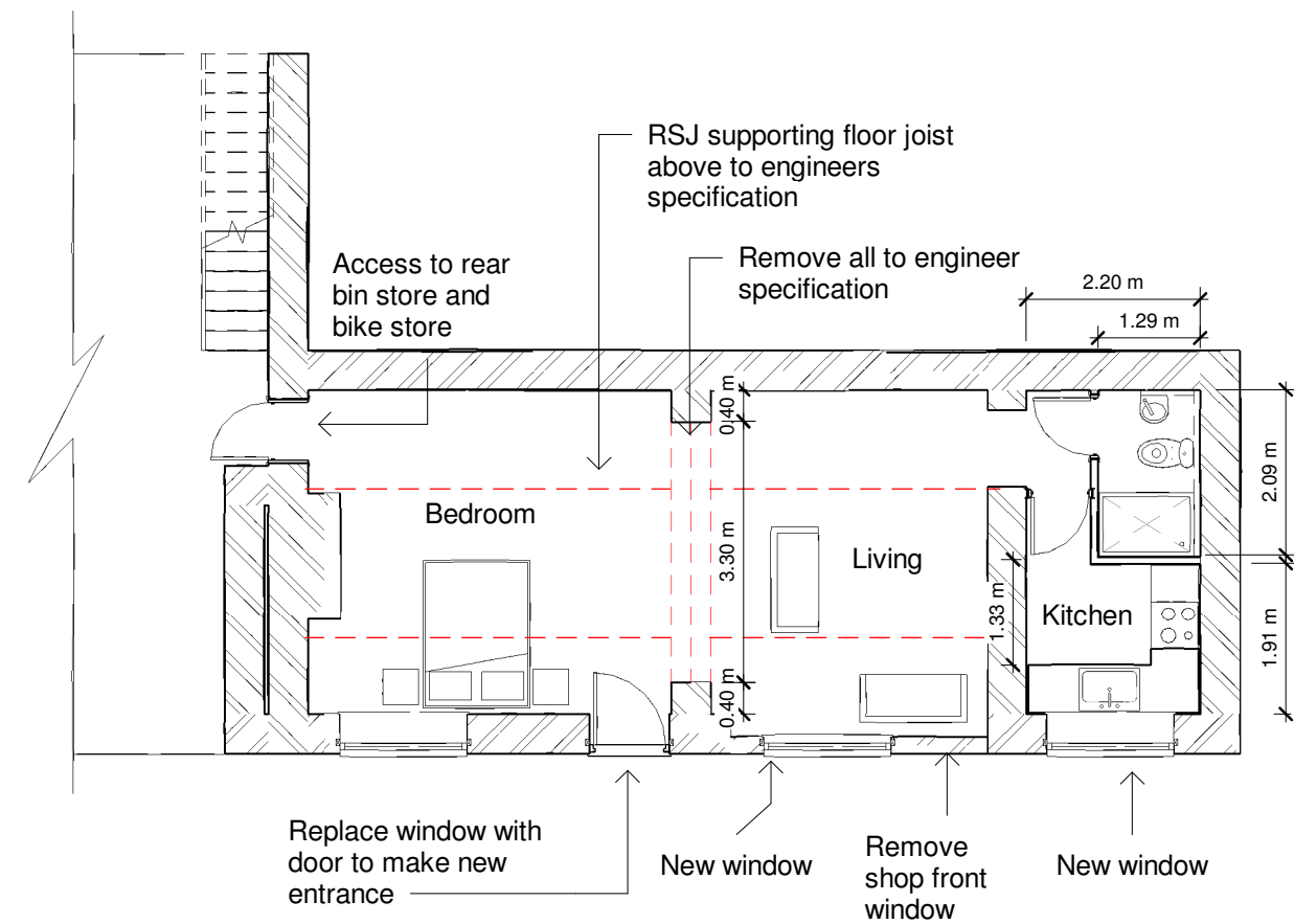
Proposed GF 1 : 100
