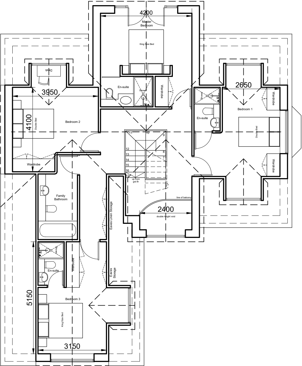
Proposed First Floor Plan A3 @ 1:100
