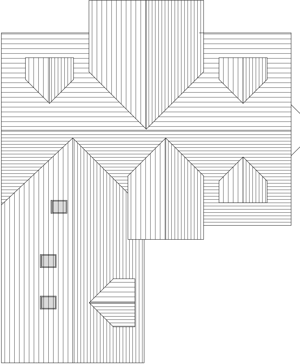
Proposed Roof Plan A3 @ 1:100
