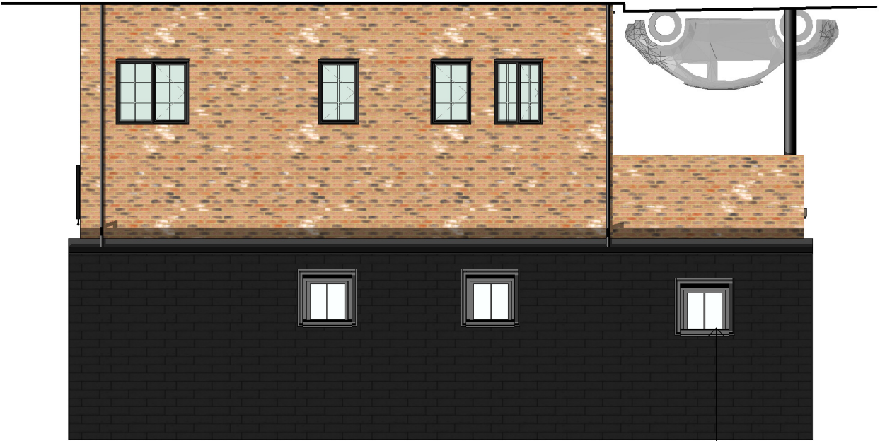
3 1 : 100 Proposed Right Elevation
