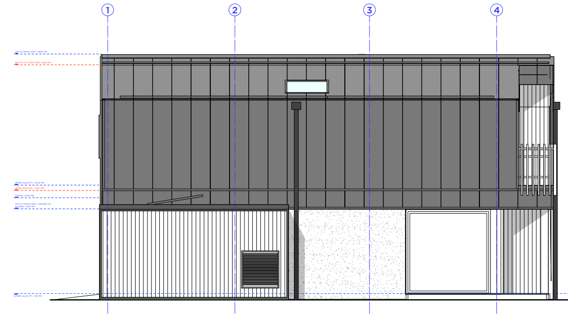
RIGHT ELEVATION | 1:25
