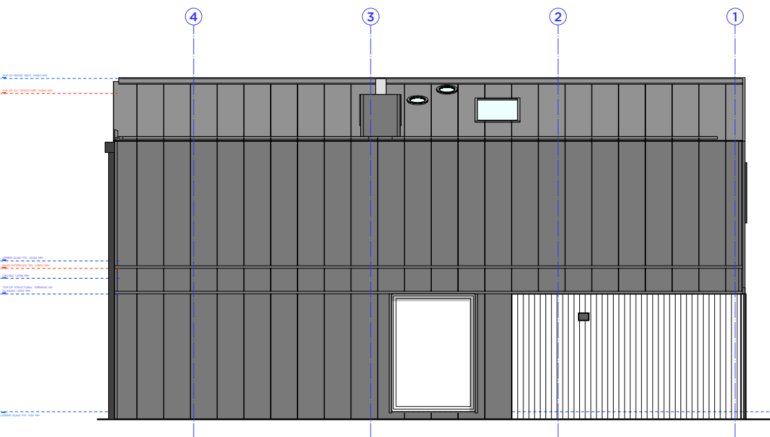
LEFT ELEVATION | 1:25
