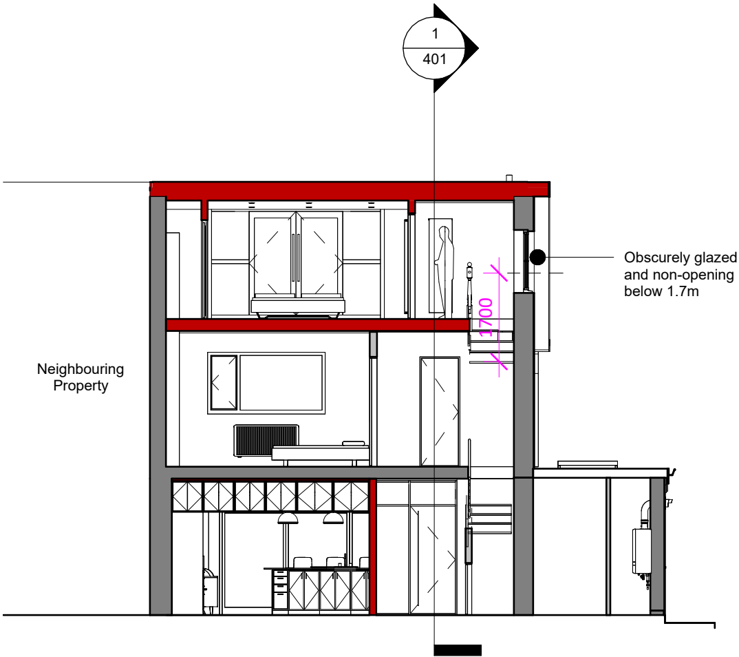
Section BB
