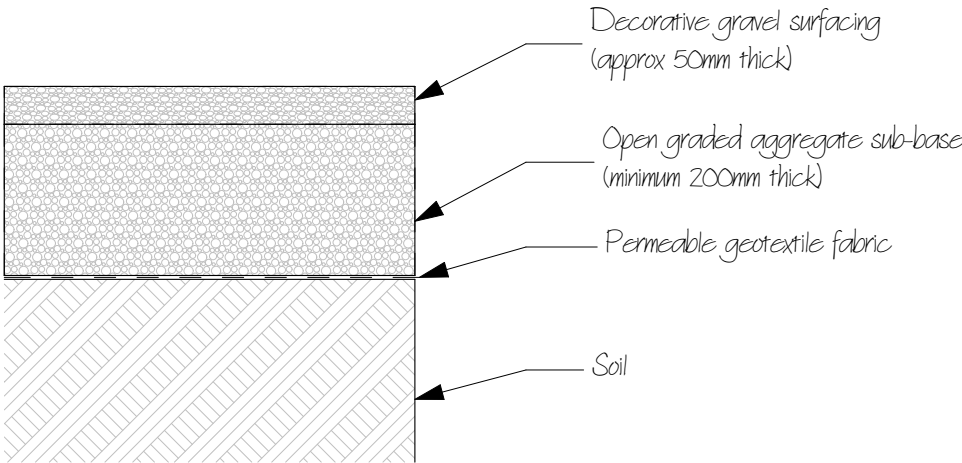
L-08 Driveway Section 1:10
