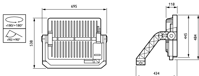
OptiVision LED gen3.5 BVP518/BVP528
