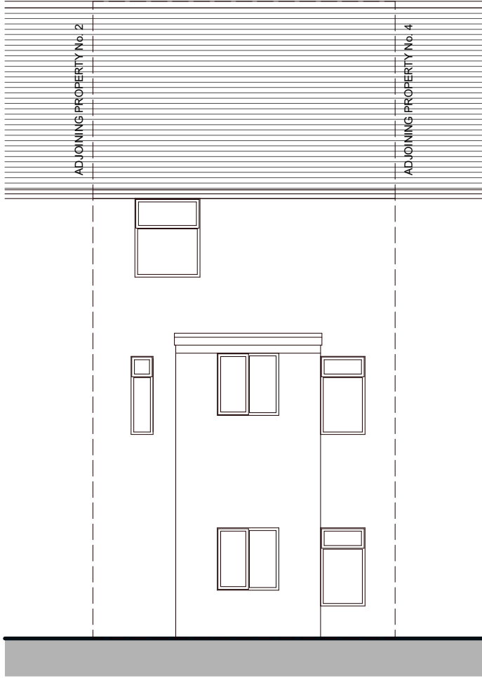
REAR ELEVATION
