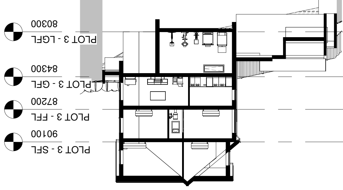
SECTION 3
