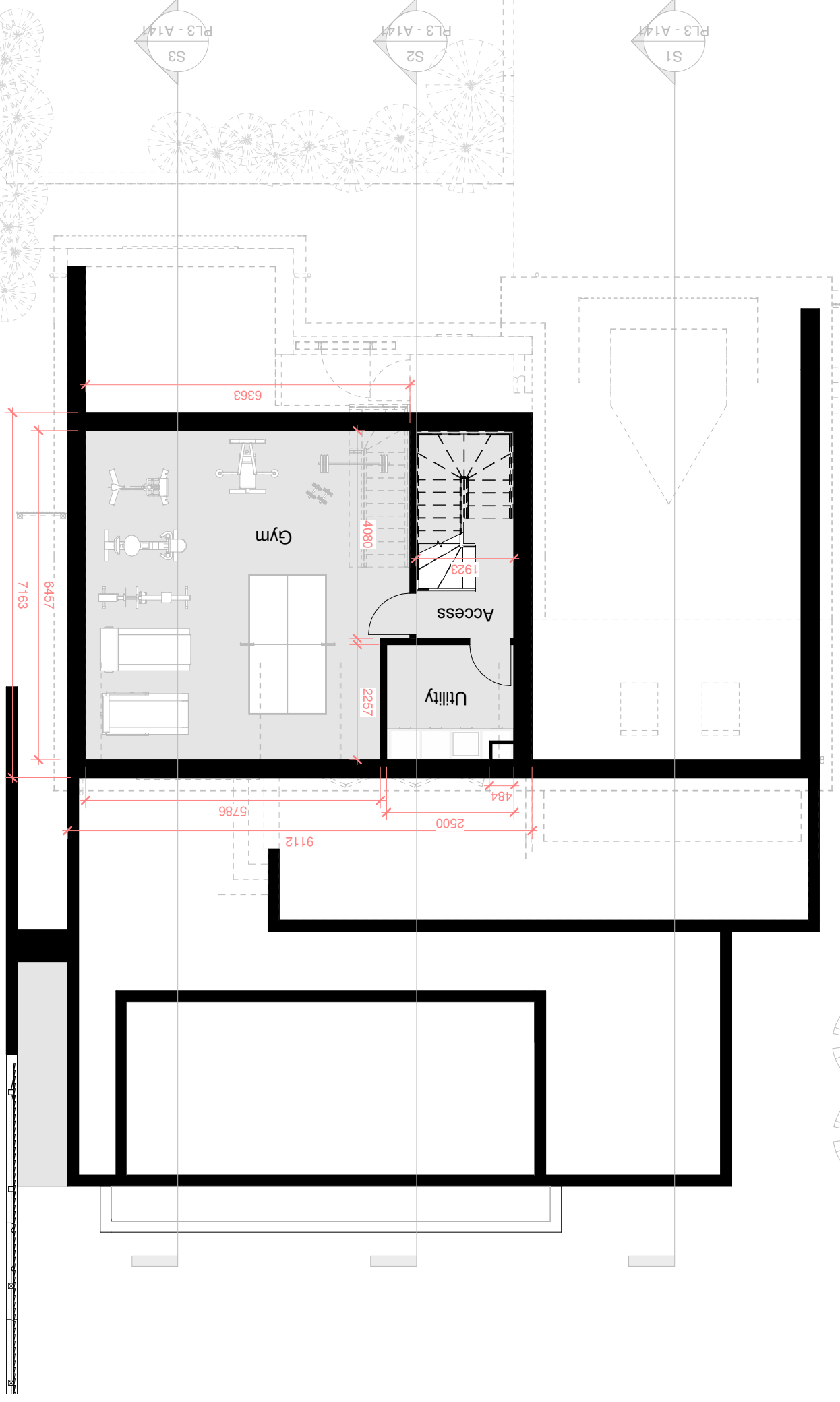
PLOT 3 - LGFL 1 : 100
