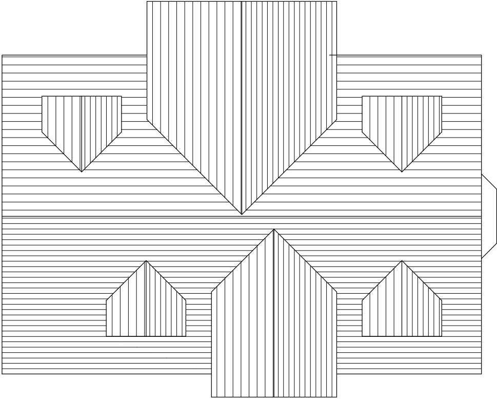
Proposed Roof Plan A1 @ 1:50
