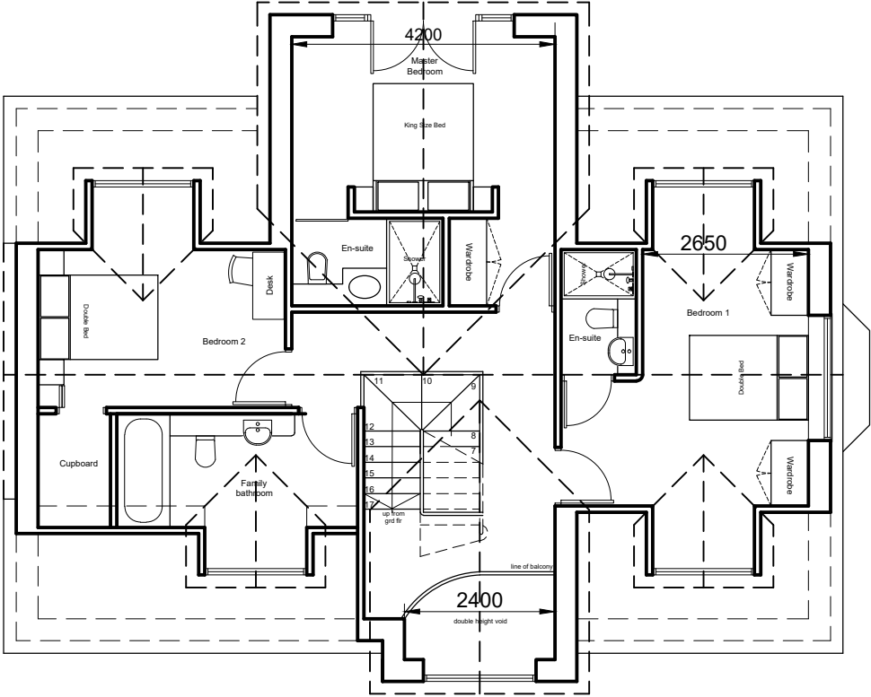
Proposed First floor plan A1 @ 1:50
