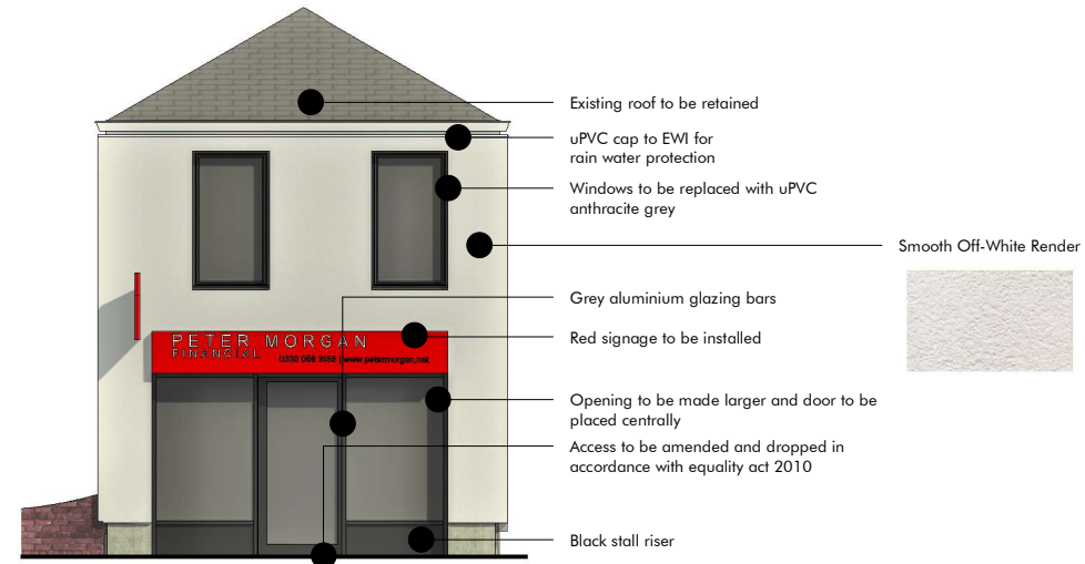
1:100 Proposed Front Elevation
