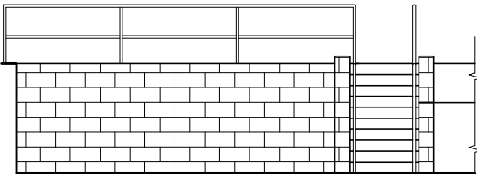
Retaining Wall / Steps Elevation
