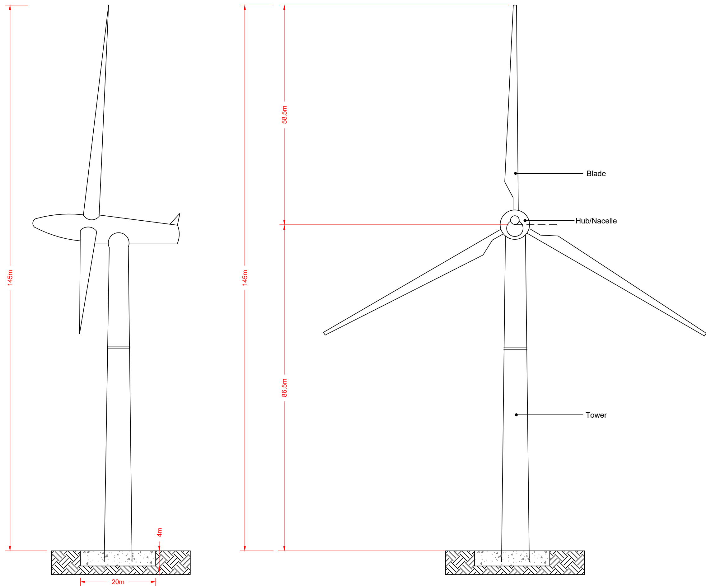
Figure 5.3b Wind turbine elevations - 58.5m blade length (117m rotor diameter)
