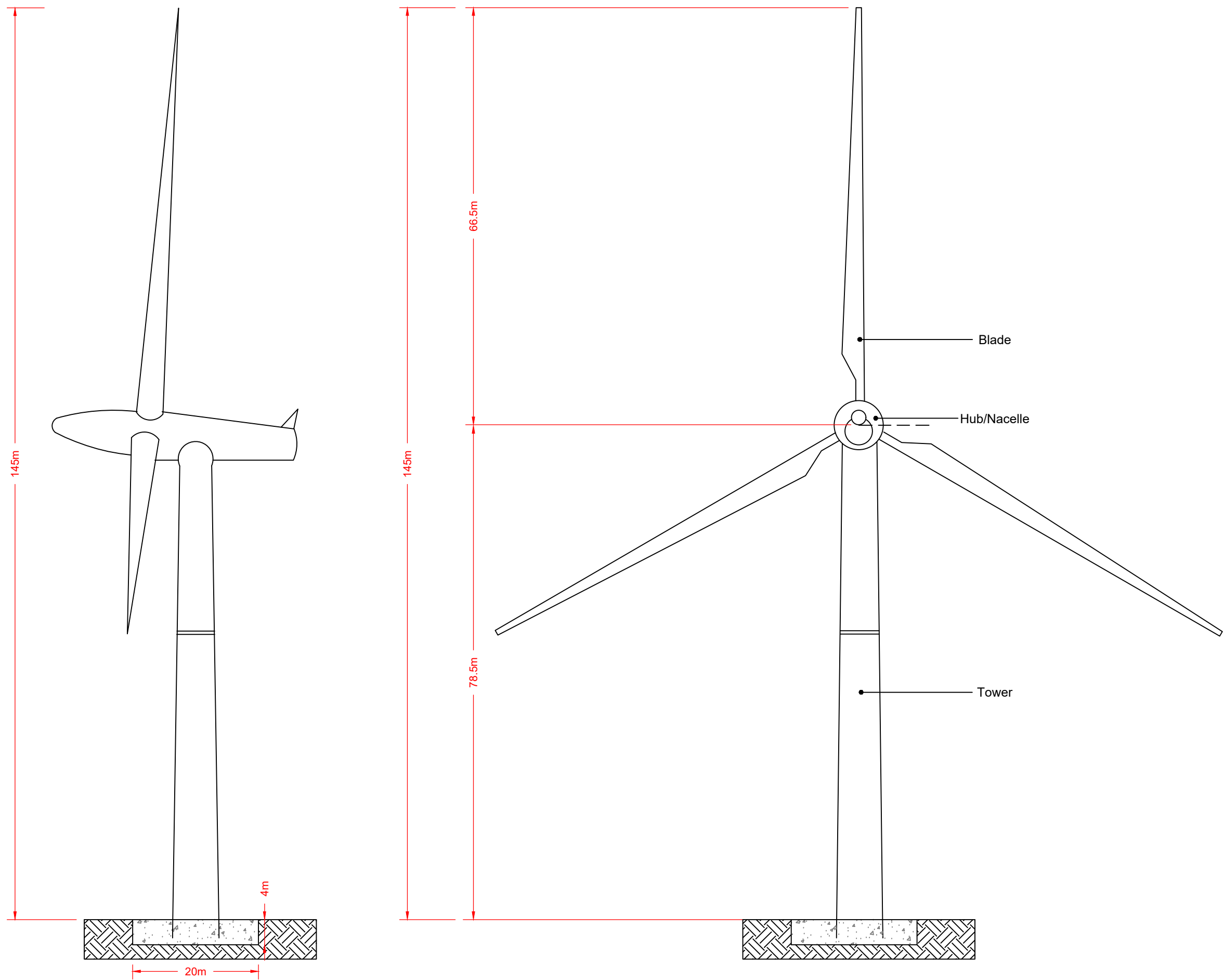
Figure 5.3a Wind turbine elevations - 66.5m blade length (133m rotor diameter)
