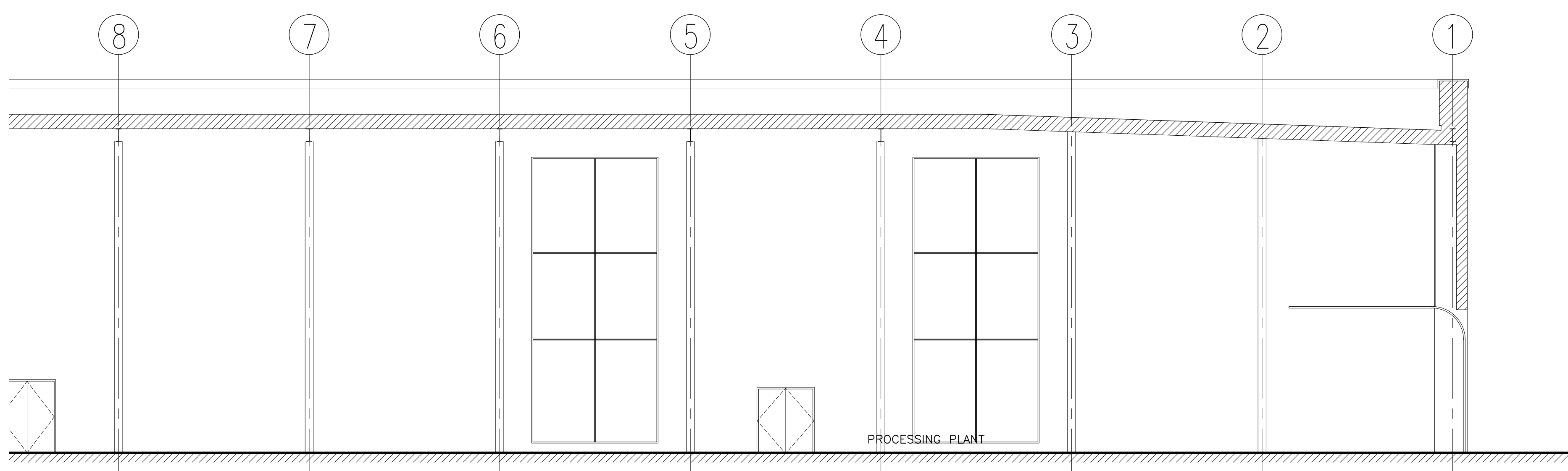
SECTION E - E (VIEW 03) VIEW TO GRID LINE D SCALE 1:100 @ A0
