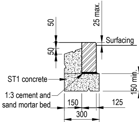
PROPOSED BN DROPPED (DK) KERB DETAIL
