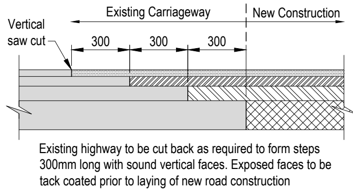
PROPOSED ASHPALT PARKING BAY EXISTING CARRIAGEWAY TIE IN DETAIL
