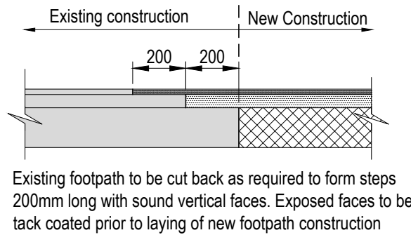
PROPOSED ASPHALT CYCLE TRACK / FOOTWAY TIE IN DETAIL
