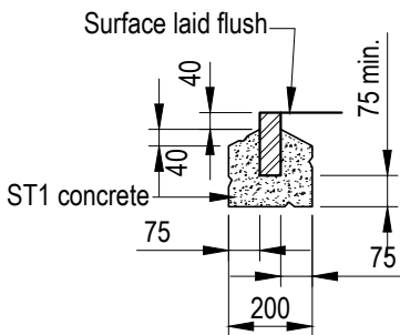
PROPOSED EF KERB DETAIL
