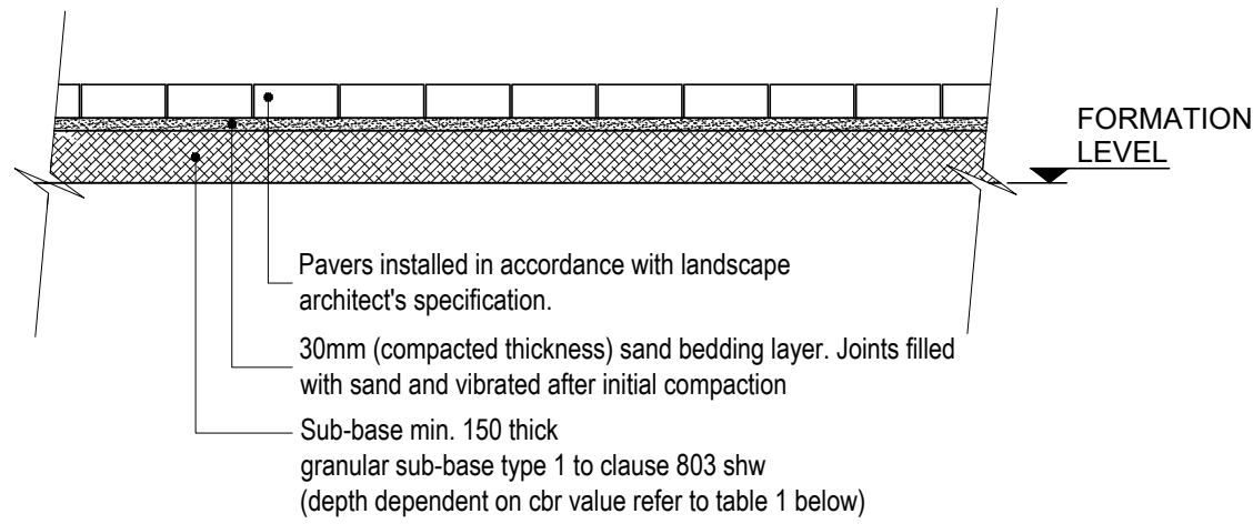
PROPOSED PAVED AREAS CONSTRUCTION DETAIL
