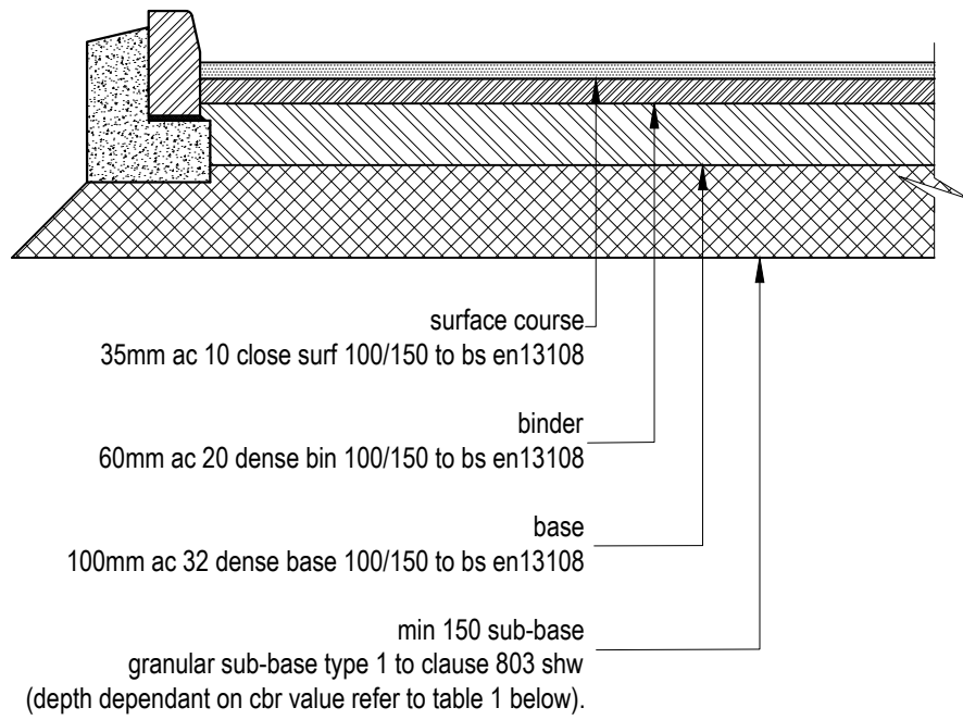
PROPOSED ASPHALT PARKING BAY CONSTRUCTION DETAIL
