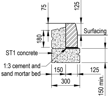
PROPOSED HB2 KERB DETAIL
