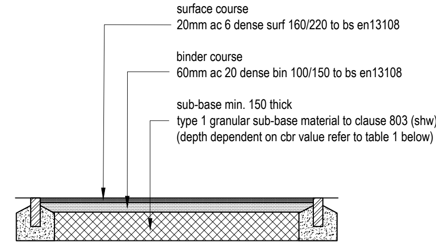
PROPOSED ASPHALT CYCLE TRACK / FOOTWAY CONSTRUCTION DETAIL
