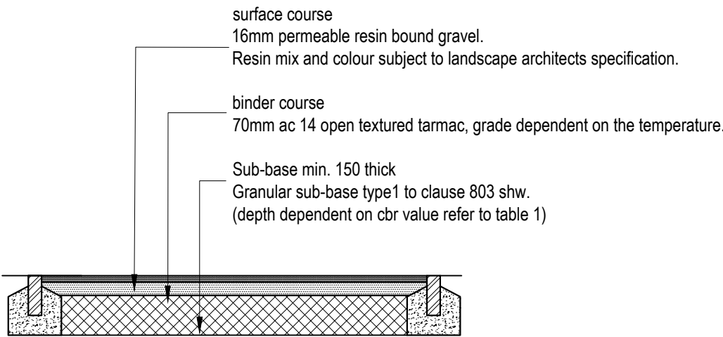
RESIN BOUND GRAVEL FOOTWAY CONSTRUCTION DETAIL
