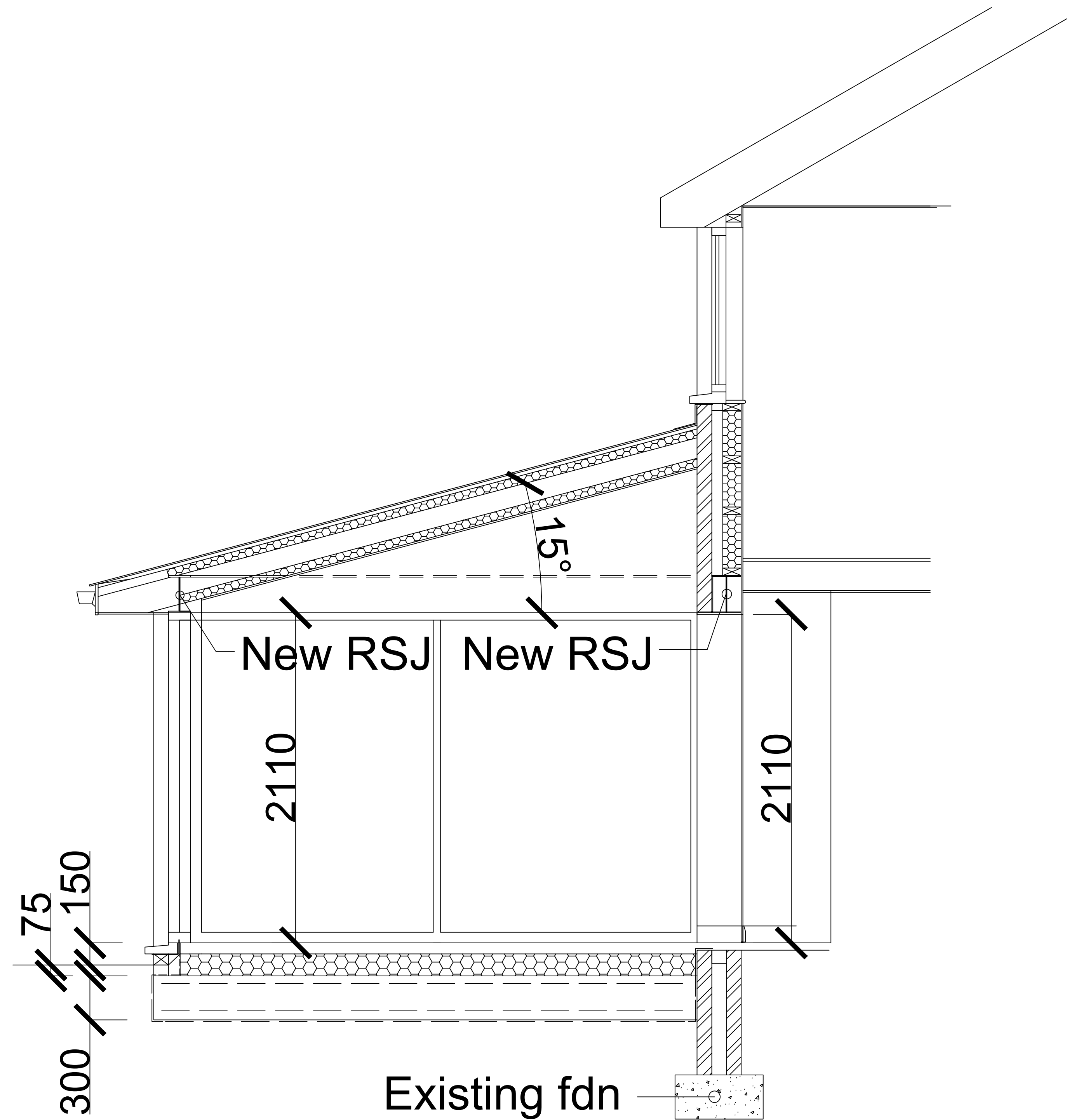
PROPOSED SECTION A-A
