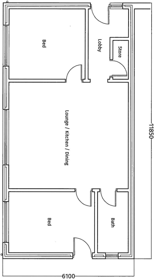
Existing Floor Plan 1:100 (at A4)
