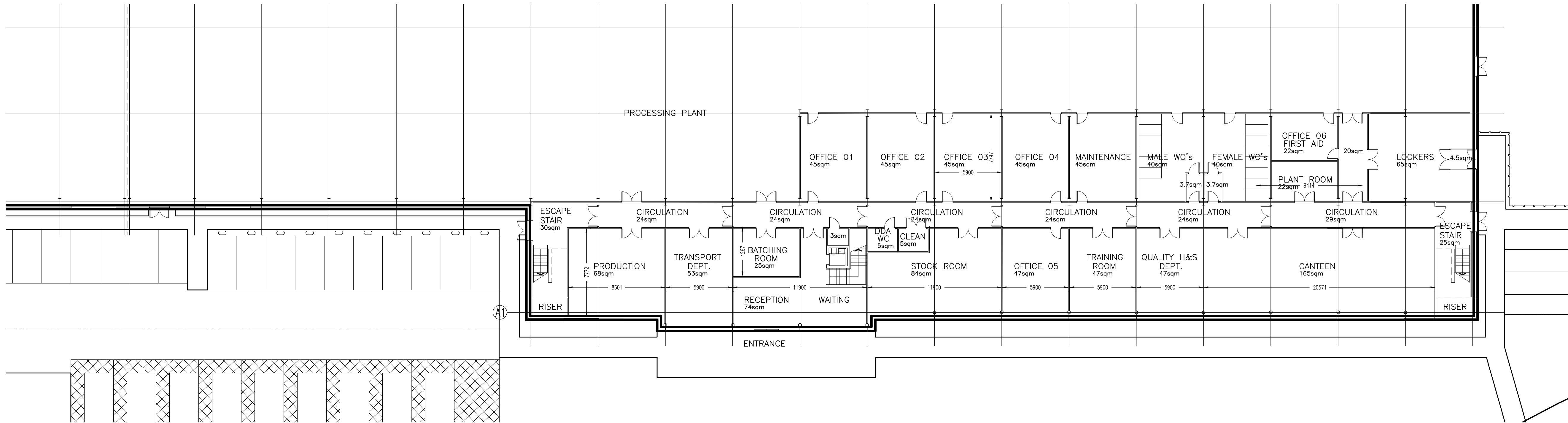
GROUND FLOOR – ADMINISTRATION AND STAFF ACCOMMODATION
