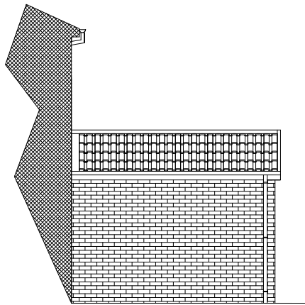
Proposed Side Elevation (Viewed from No17)
