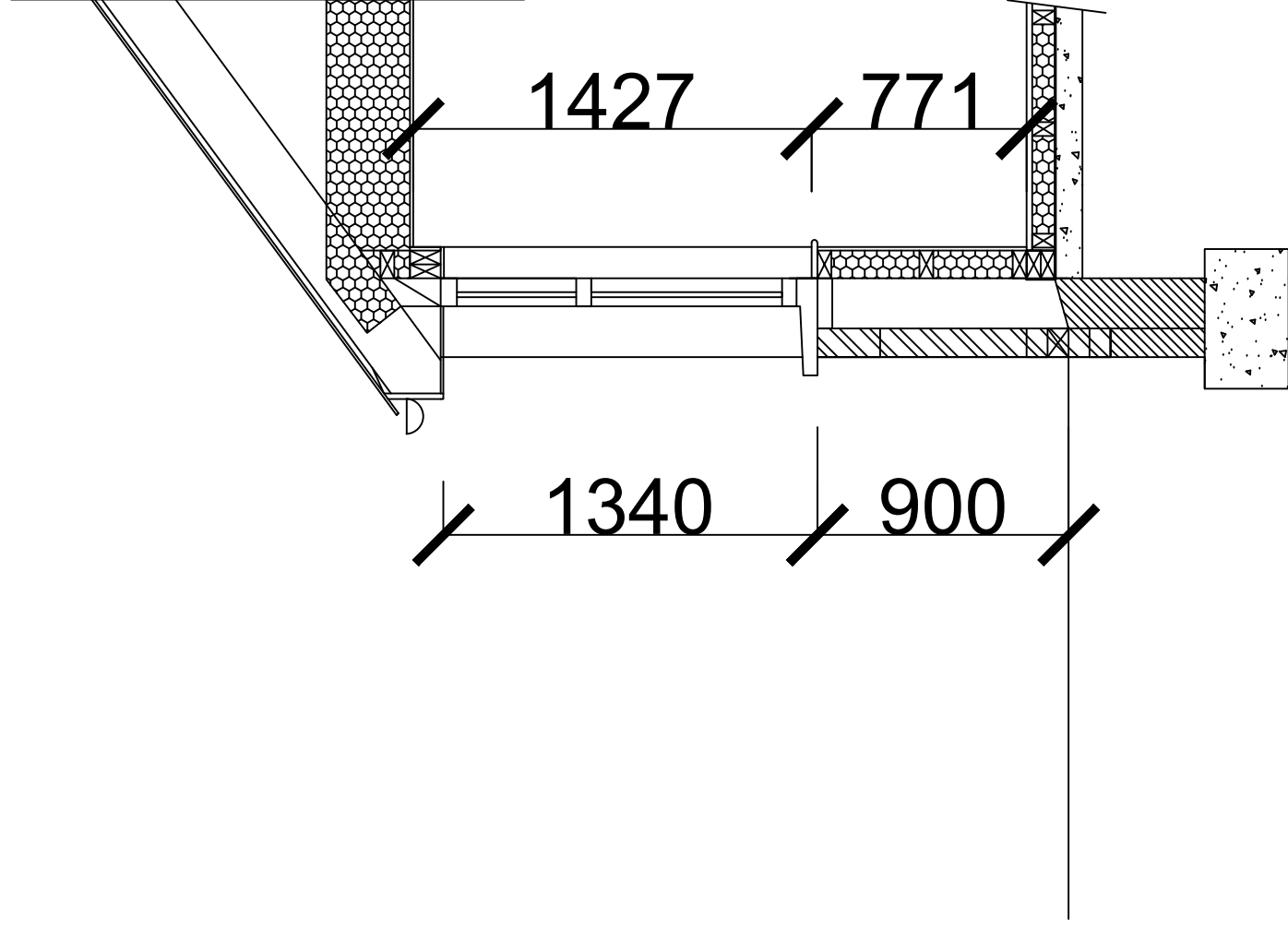
SECTION B-B Drg. No. B-04 Scale 1:25
