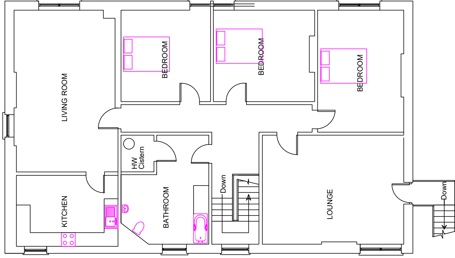
EXISTING PLAN OF 2ND FLOOR FLAT
