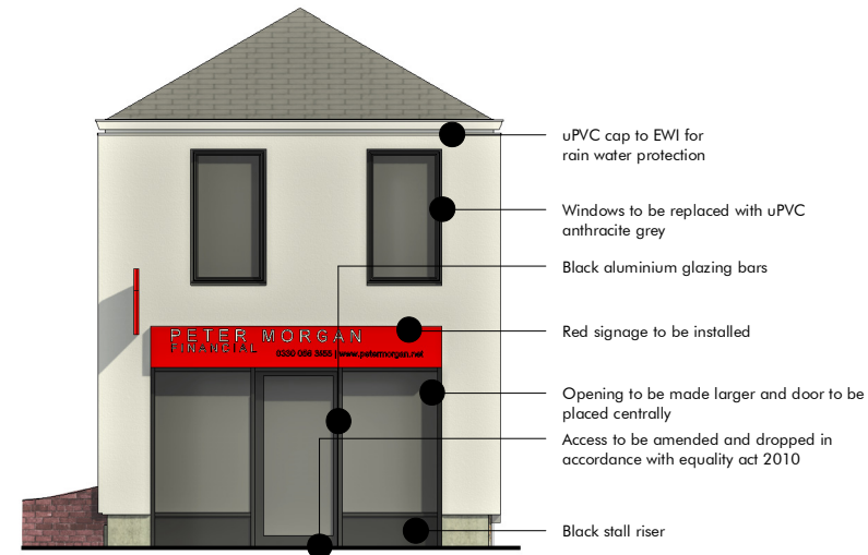
1:100 Proposed Front Elevation
