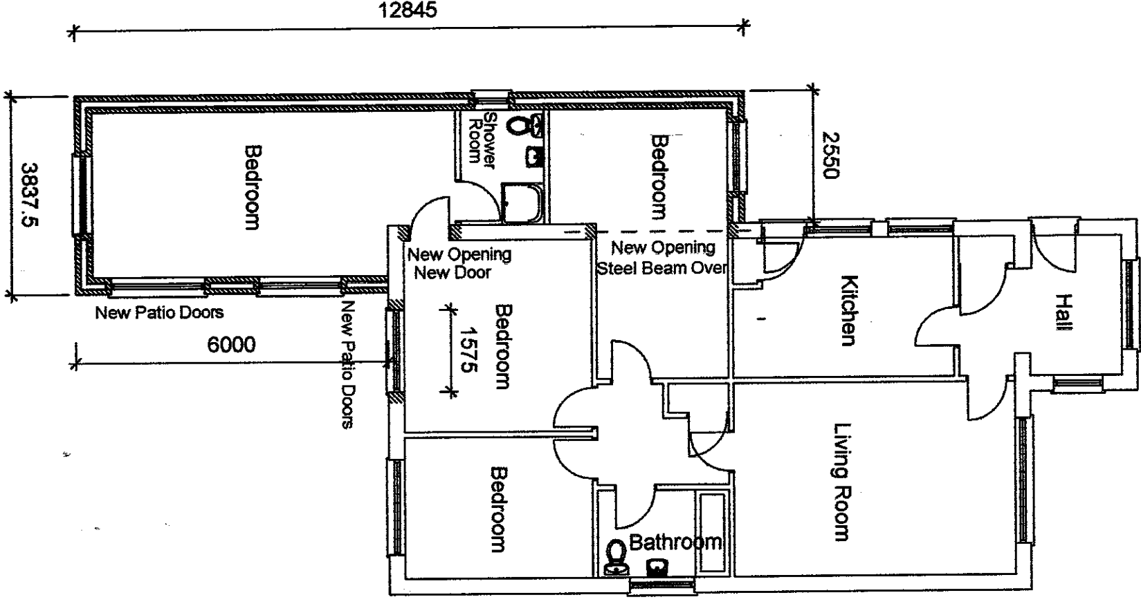
Ground Floor Plan as Proposed
