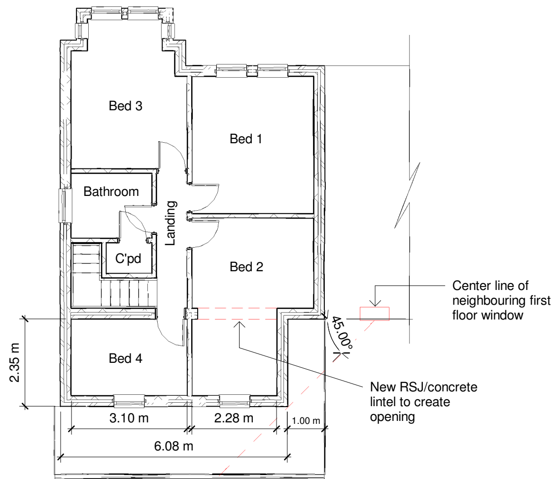
Proposed FF 1 : 100
