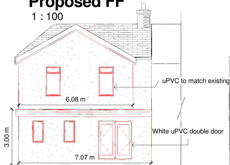
Proposed Rear 1 : 100
